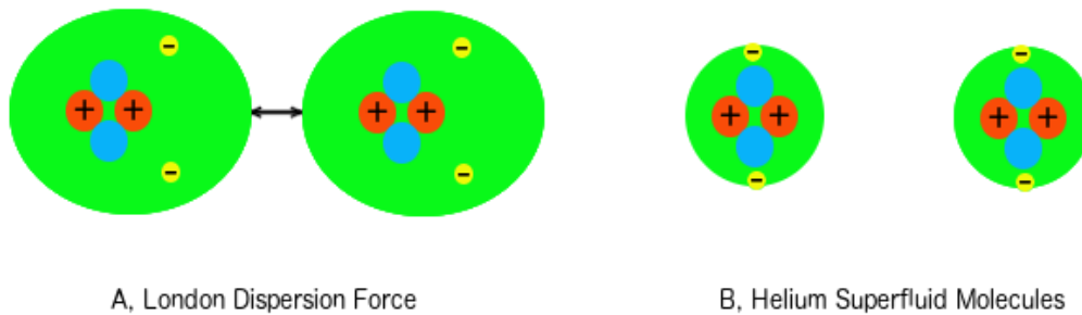
Figure 4: The vanishing of intermolecular attraction and viscosity in superfluids. A) Due to the single fully occupied valence orbital in helium atoms, there are no other interactions between helium molecules except for London dispersion forces, contributing to the viscosity of helium liquids. B) At low temperatures, electrons retreat to lower orbitals, reducing their dispersion and eventually leading to the disappearance of intermolecular attractions.
