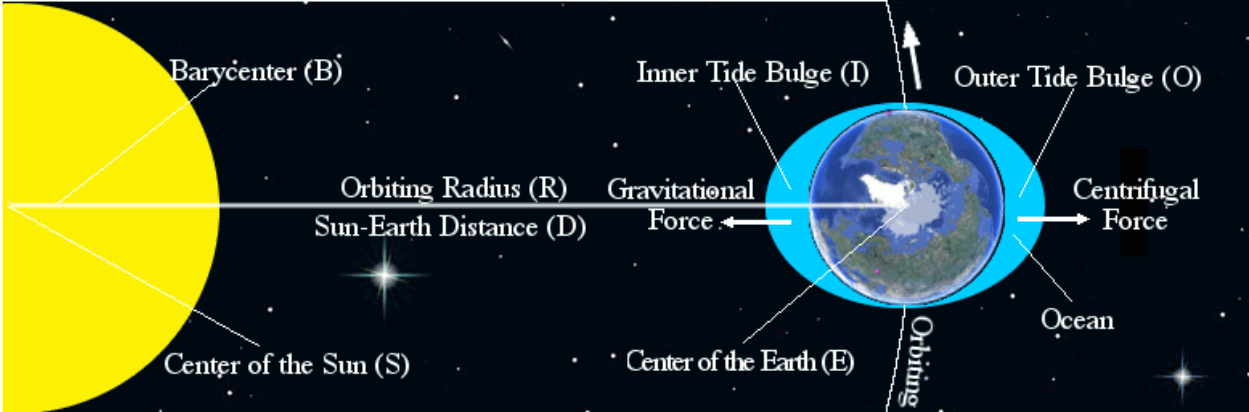
Figure 1, Formation of tides.
